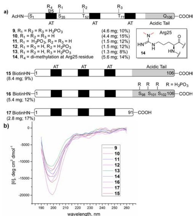
Figure 3. (a) Synthetic HMGA1a proteins (total amount and overall yields after HPLC isolation in parentheses). (b) Circular dichroism spectra of synthetic HMGA1a proteins.
