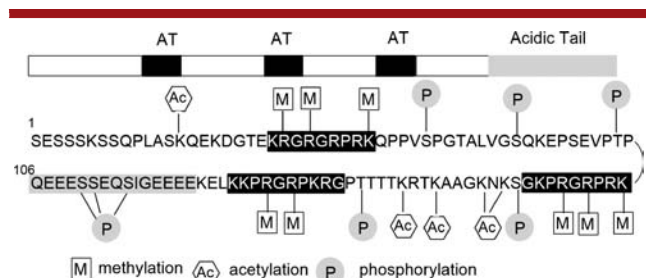
Figure 1. HMGA1a with diverse post-translational modifications.
