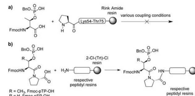
Scheme 2. (a) Fmoc-Thr(HPO 3 Bn)-OH Failed To Be Incorporated during SPPS. (b) Fmoc-pTP-OH and Fmoc-pSP-OH Dipeptide Building Blocks Were Utilized to Overcome the Difficulty of SPPS
