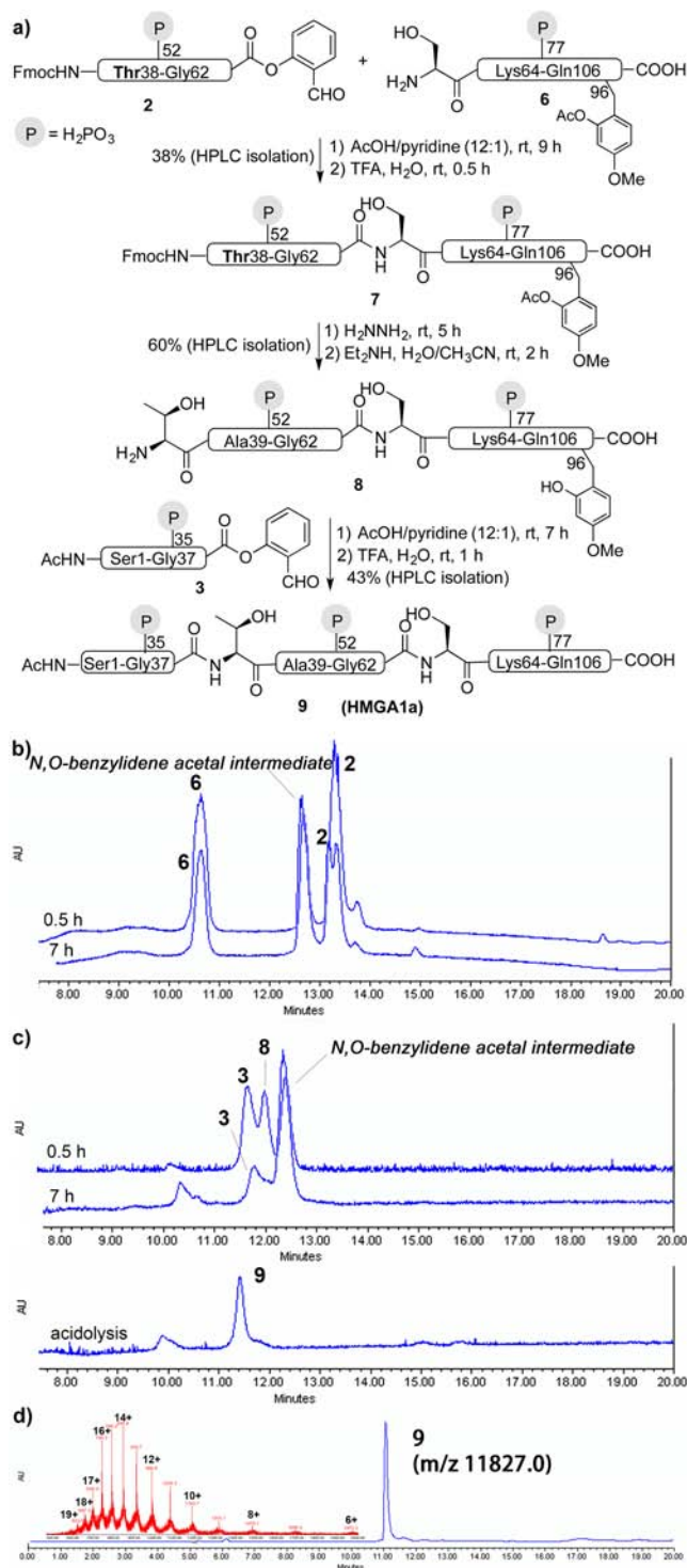
Figure 2. (a) Synthetic scheme of full-length HMGA1a. (b) Representative HPLC profile of the first ligation. (c) Representative HPLC profile of the second ligation. (d) HPLC-MS characterization of the purified final product HMGA1a 9.
