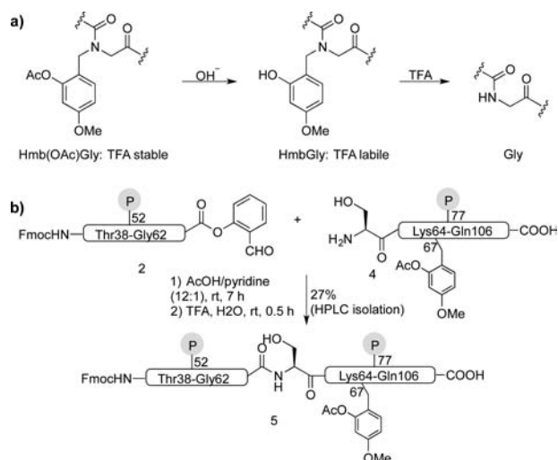
Scheme 3. (a) Backbone Hmb Protection. (b) Hmb Served To Improve Ligation Efficiency
