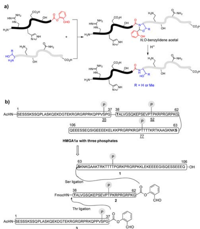
Scheme 1. (a) Ser/Thr ligation (STL). (b) Retrosynthetic Plan of HMGA1a According to the Principle of STL
